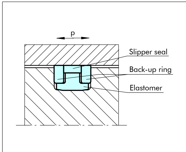
Figure 20 PHD Seal
