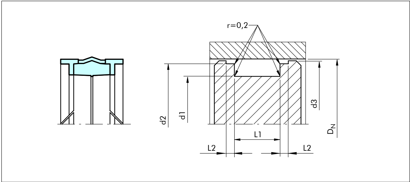
Figure 50 Installation drawing
