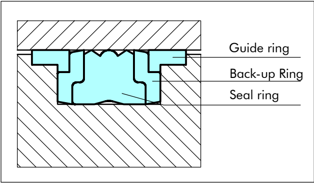
Figure 40 D-A-S Compact Seal, Type B
