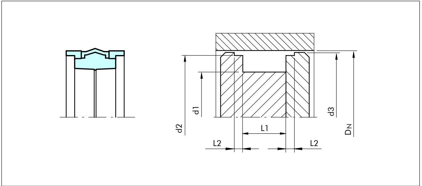
Figure 51 Installation drawing
