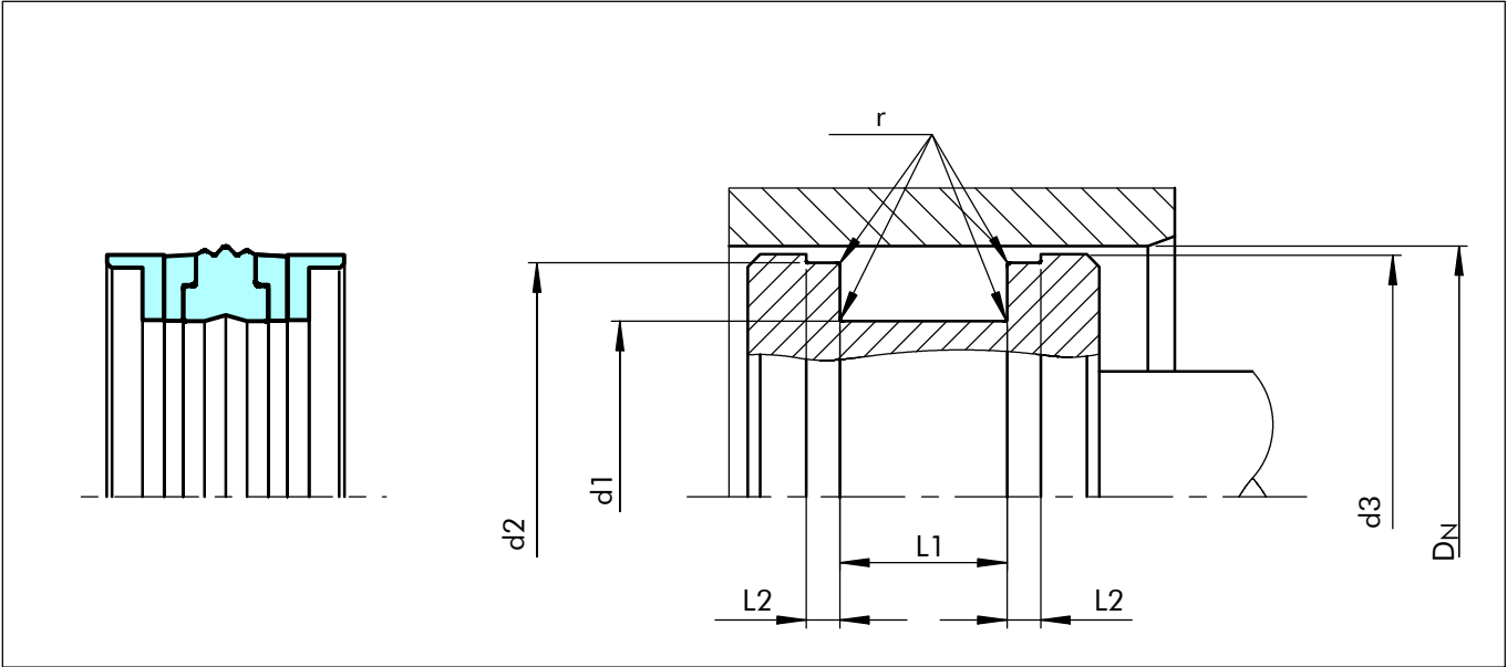
Figure 42 Installation drawing
