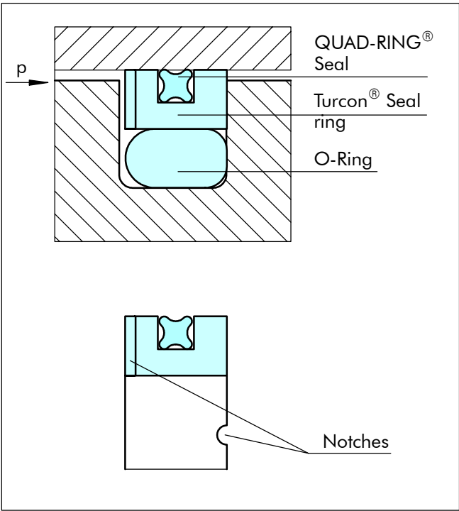
Figure 18 Turcon® AQ-Seal®
