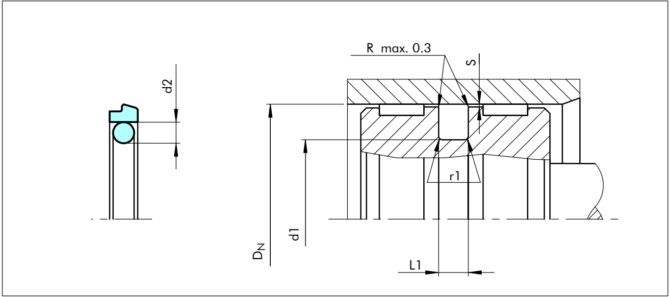
Figure 25 Installation drawing
