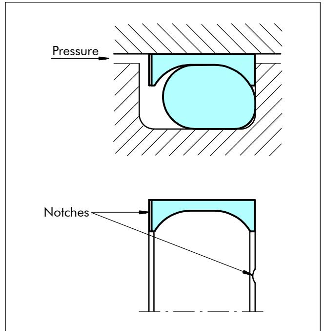
Figure 27 Turcon® Double Delta® with notches
