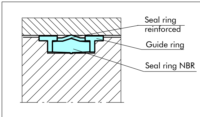
Figure 48 Compact Seal, Type DPS
