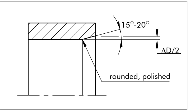
Figure 28 Lead-in chamfers
