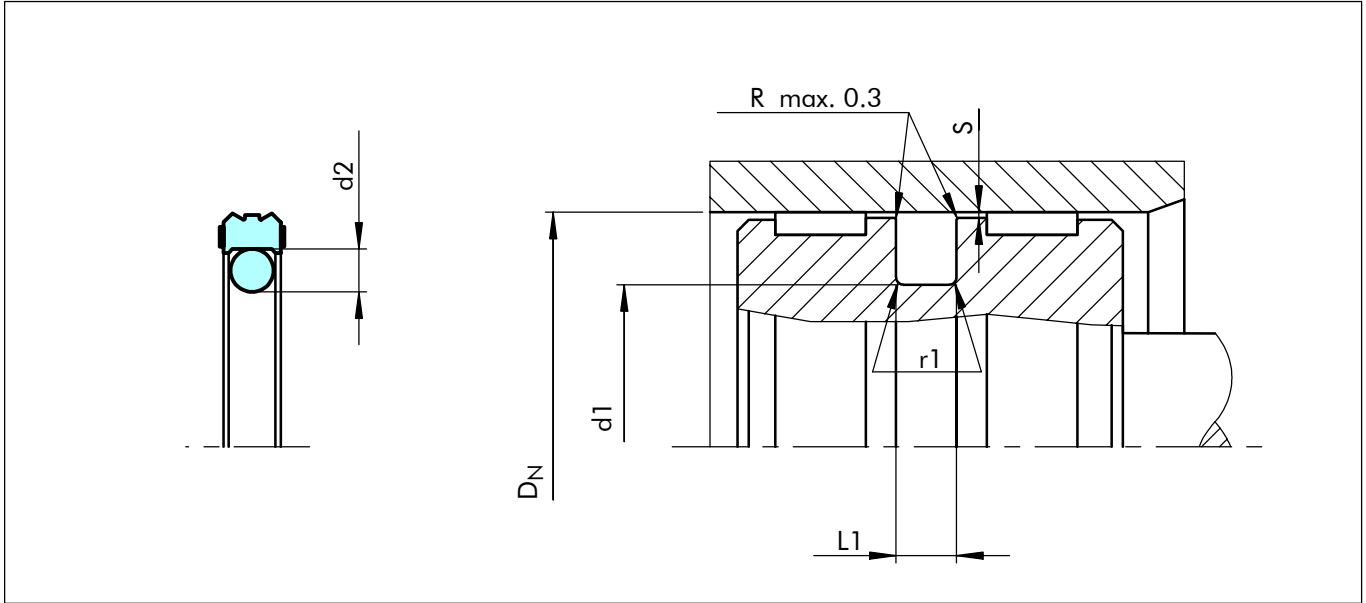
Figure 36 Installation drawing
