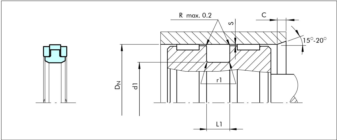
Figure 21 Installation drawing
