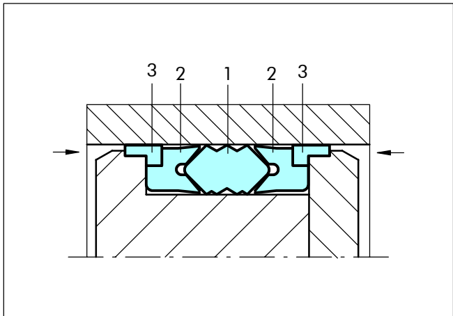
Figure 54 Selemaster design
