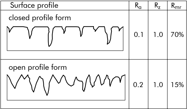
Figure 2 Profile forms of surfaces
