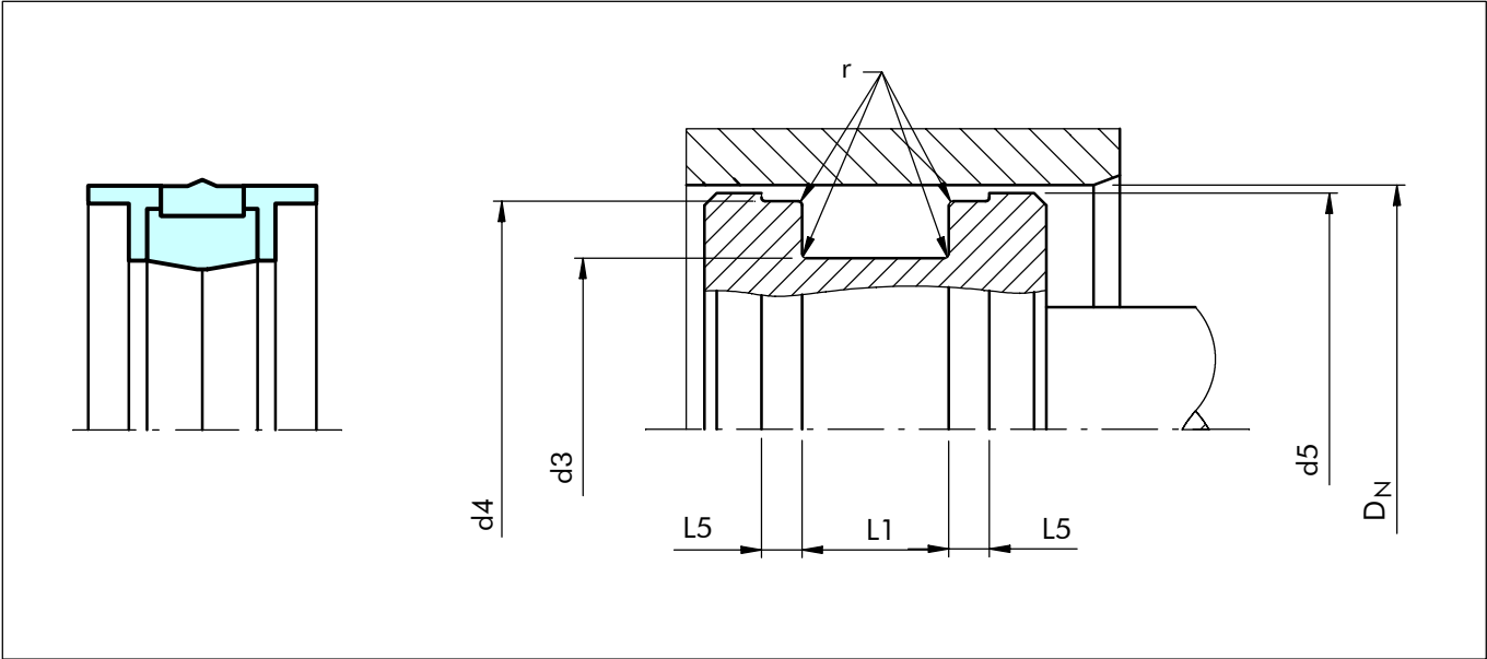
Figure 47 Installation drawing
