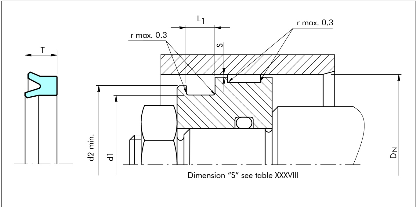
Figure 34 Installation drawing
