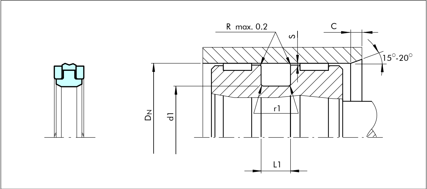
Figure 38 Installation drawing
