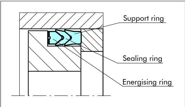
Figure 52 Veepac CH/G1
