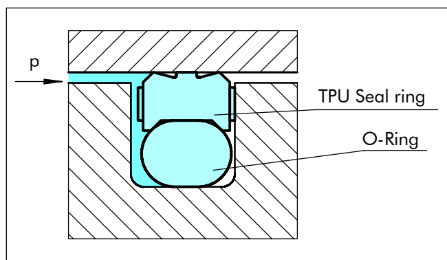
Figure 35 Zurcon ® Wynsal and GPS
