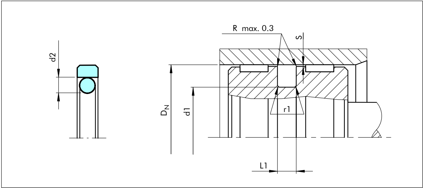
Figure 13 Installation drawing
