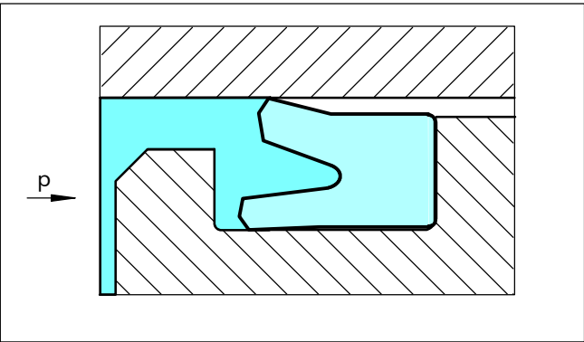
Figure 33 Piston U-Cup Type PUA and RSE
