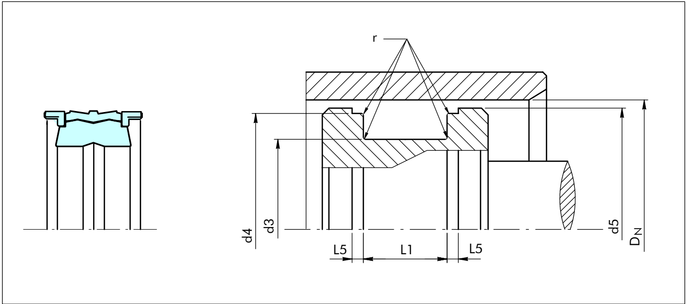
Figure 46 Installation drawing
