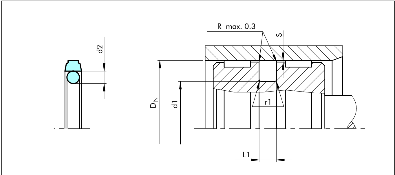
Figure 15 Installation drawing
