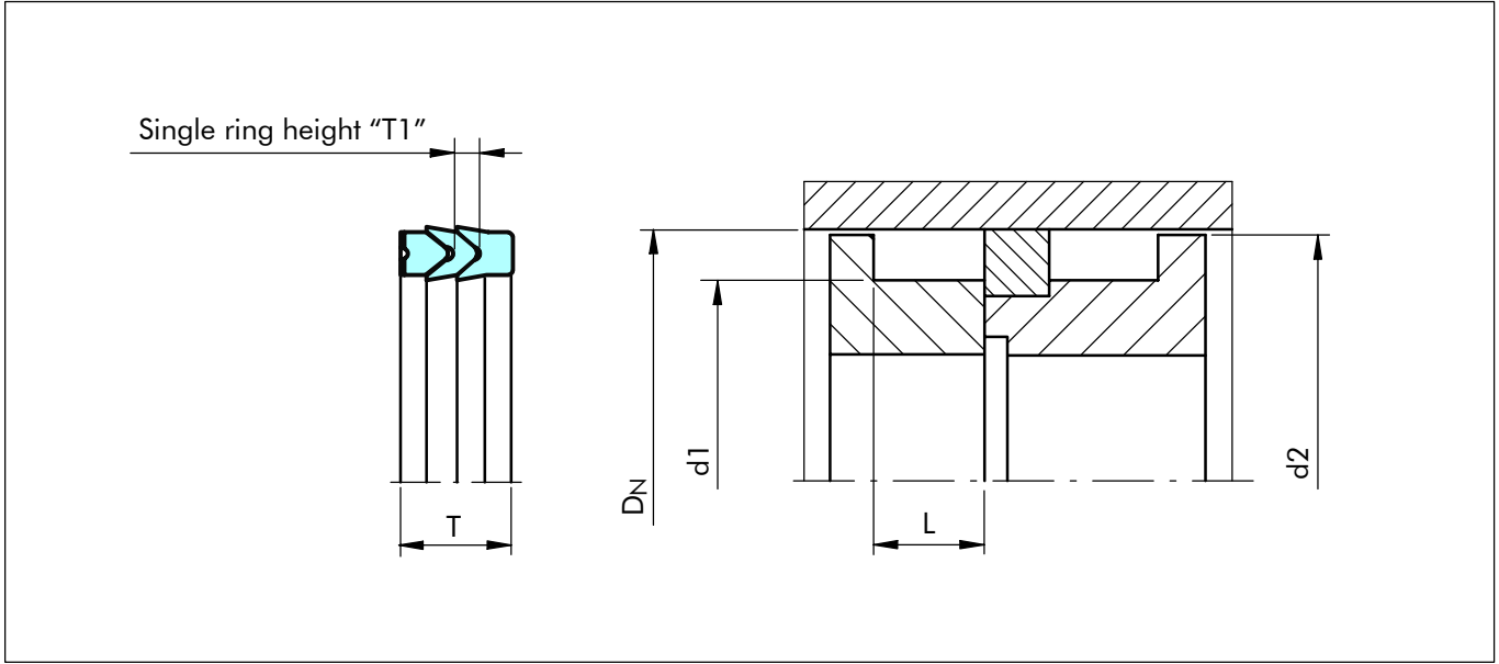
Figure 53 Installation drawing
