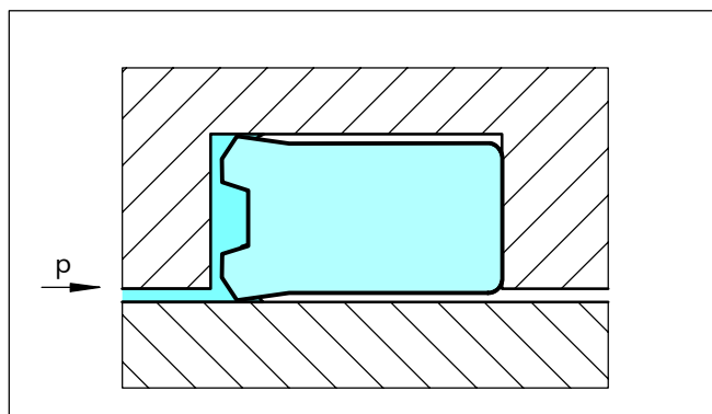
Figure 42 U-Cup, type RU1
