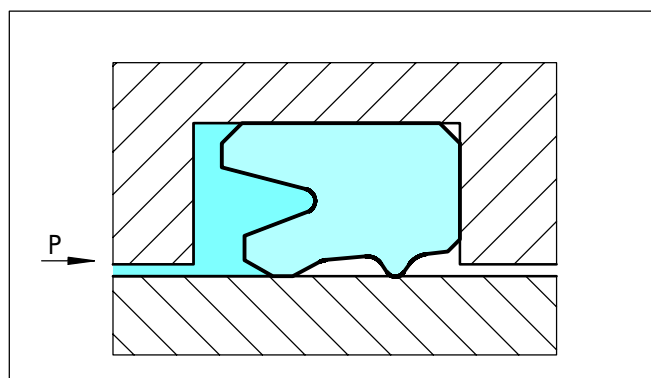
Figure 48 U-Cup, type RU3
