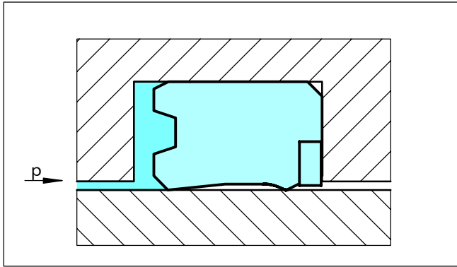
Figure 46 U-Cup, type RU2B
