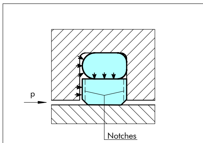
Figure 57 Turcon® Glyd Ring® with notches
