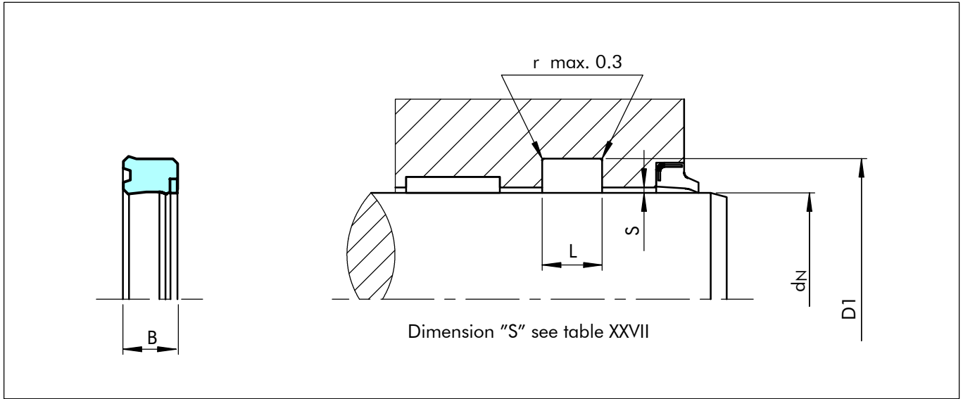
Figure 47 Installation drawing
