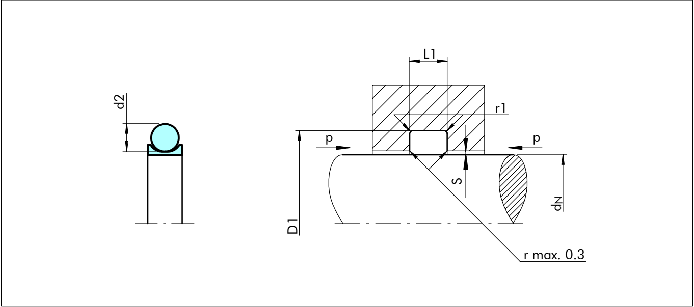
Figure 63 Installation drawing
