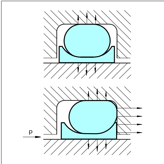
Figure 61 Turcon® Double Delta® without and with pressure
