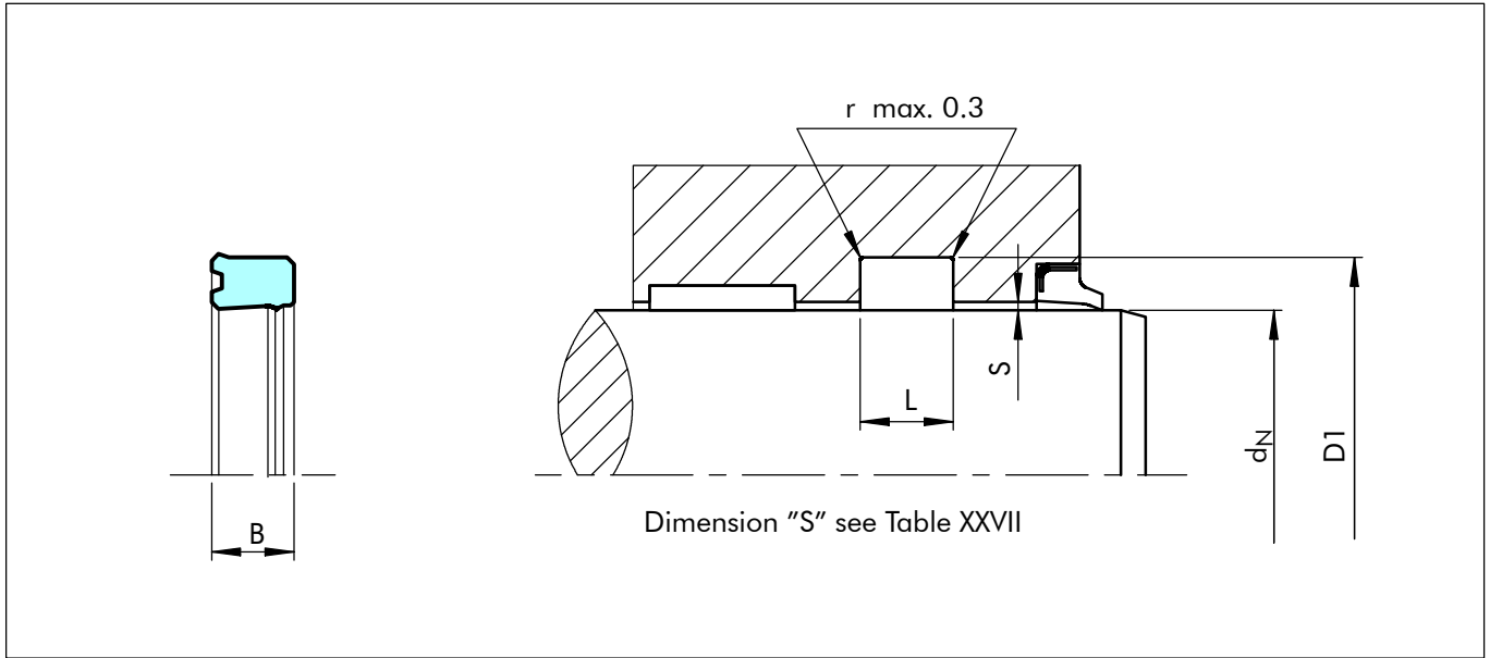
Figure 45 Installation drawing
