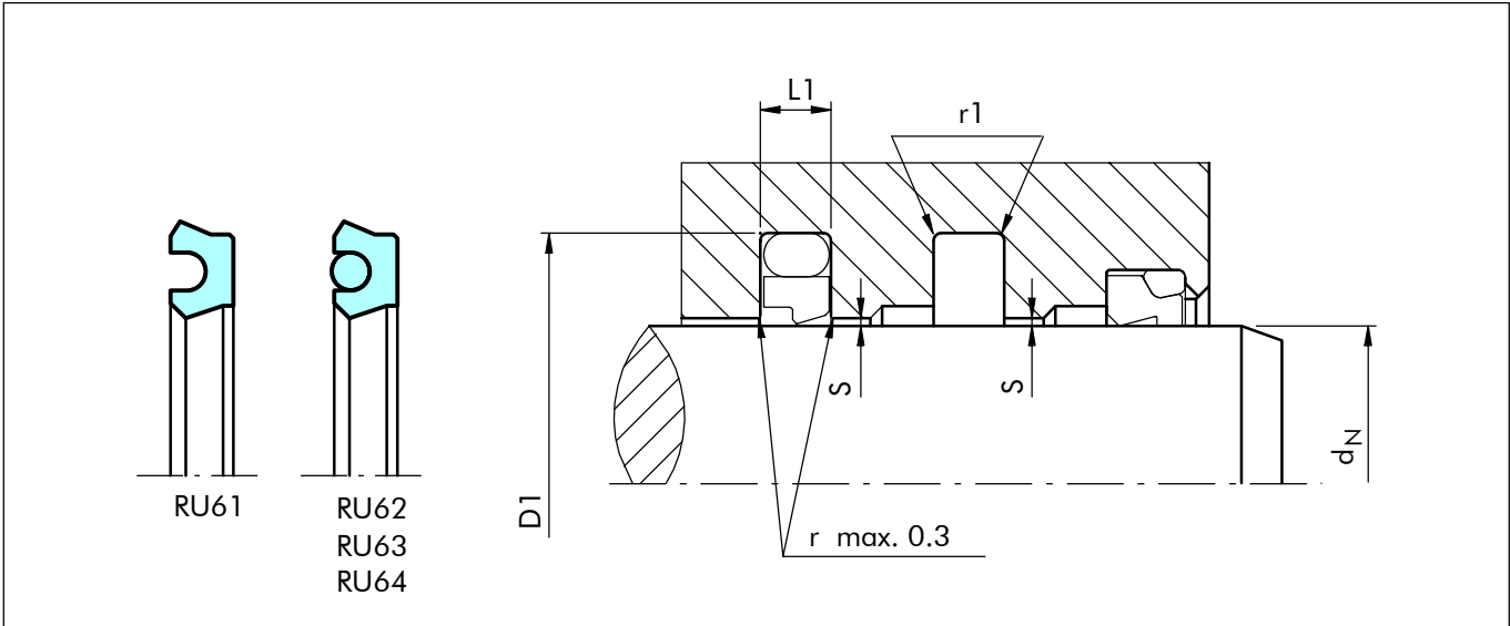
Figure 53 Installation drawing
