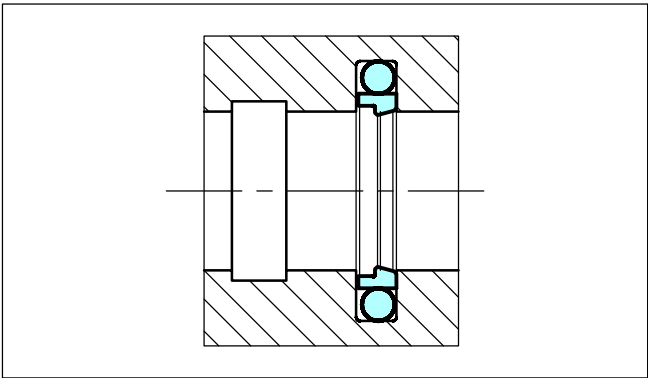
Figure 8 Installation in a closed groove
