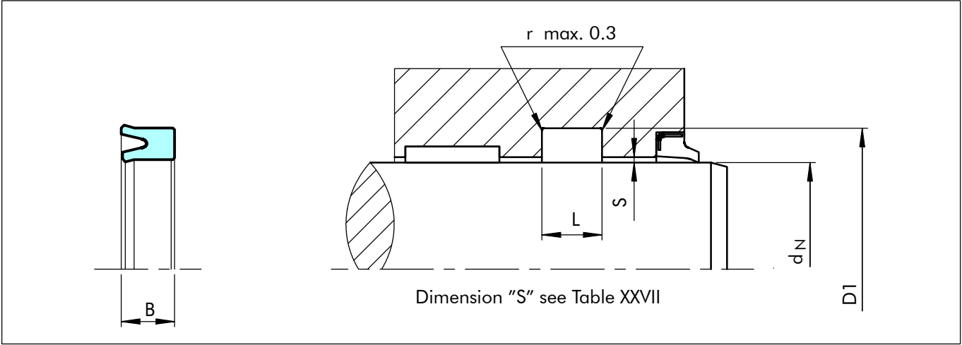
Figure 41 Installation drawing
