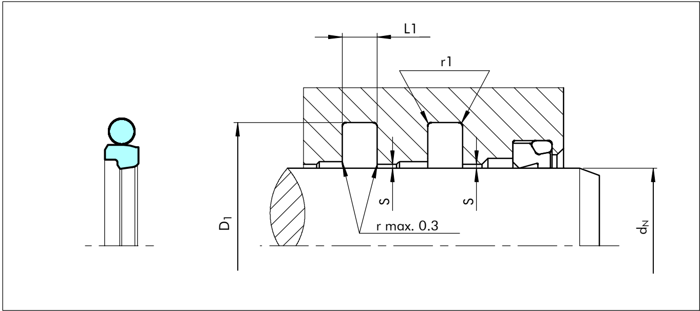
Figure 18 Installation drawing
