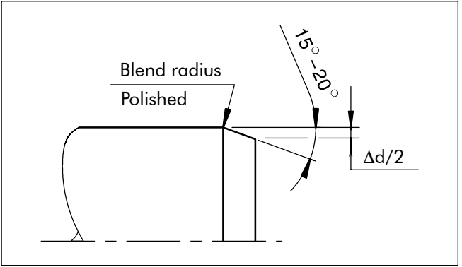
Figure 2 Lead-in chamfers
