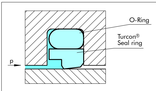
Figure 20 Turcon® Stepseal® K
