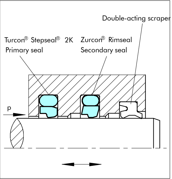
Figure 16 Turcon® Stepseal® 2K and Zurcon® Rimseal in tandem configuration
