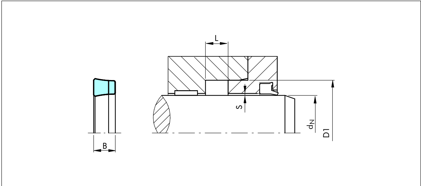
Figure 32 Installation drawing
