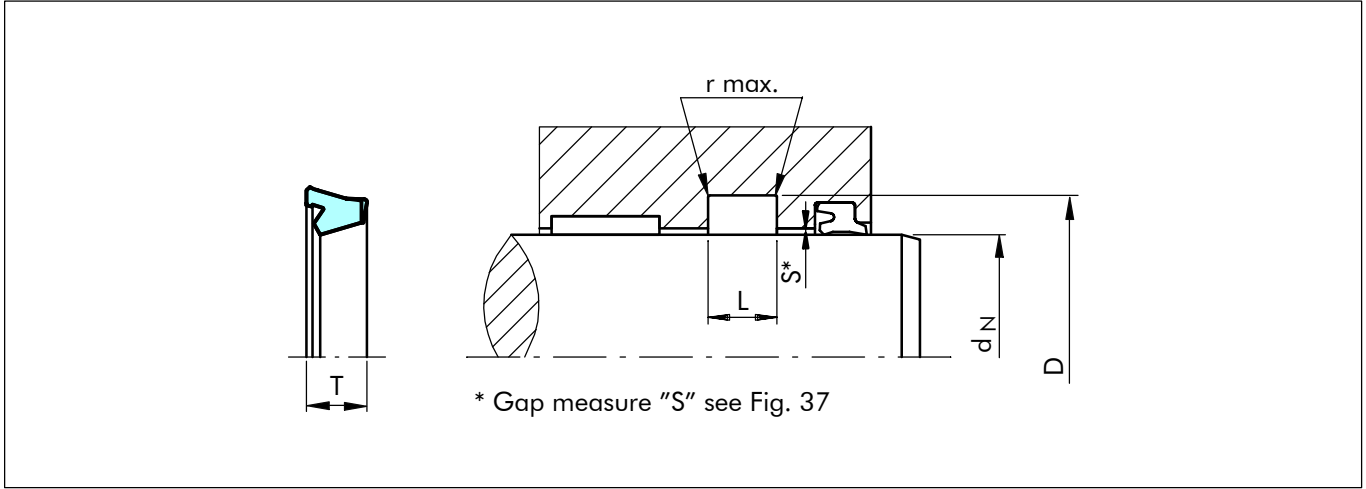
Figure 39 Installation drawing
