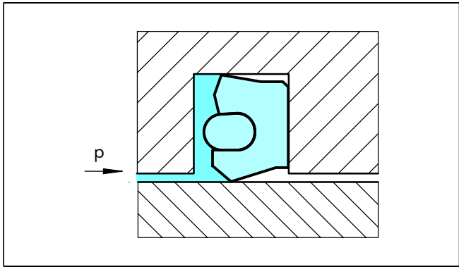
Figure 52 U-Cup, type RU6
