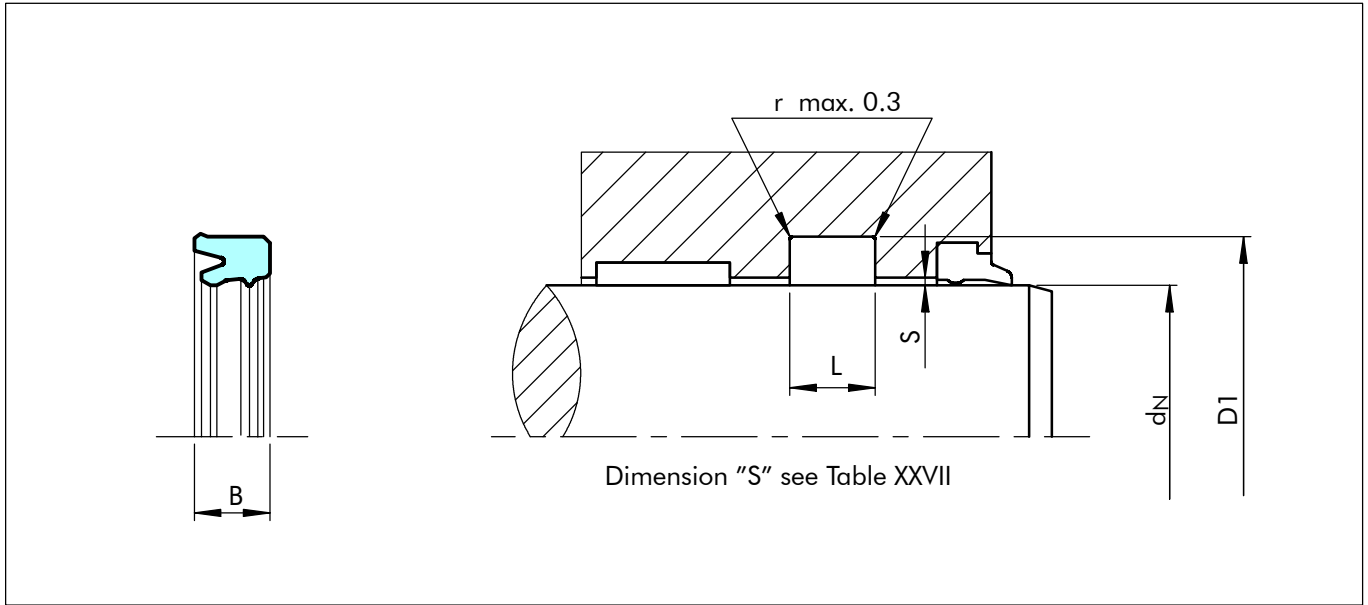
Figure 49 Installation drawing
