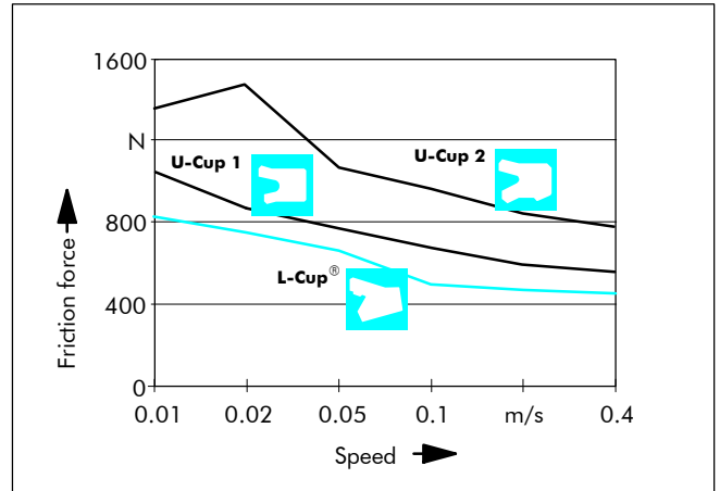
Figure 35 Friction dependent on speed
