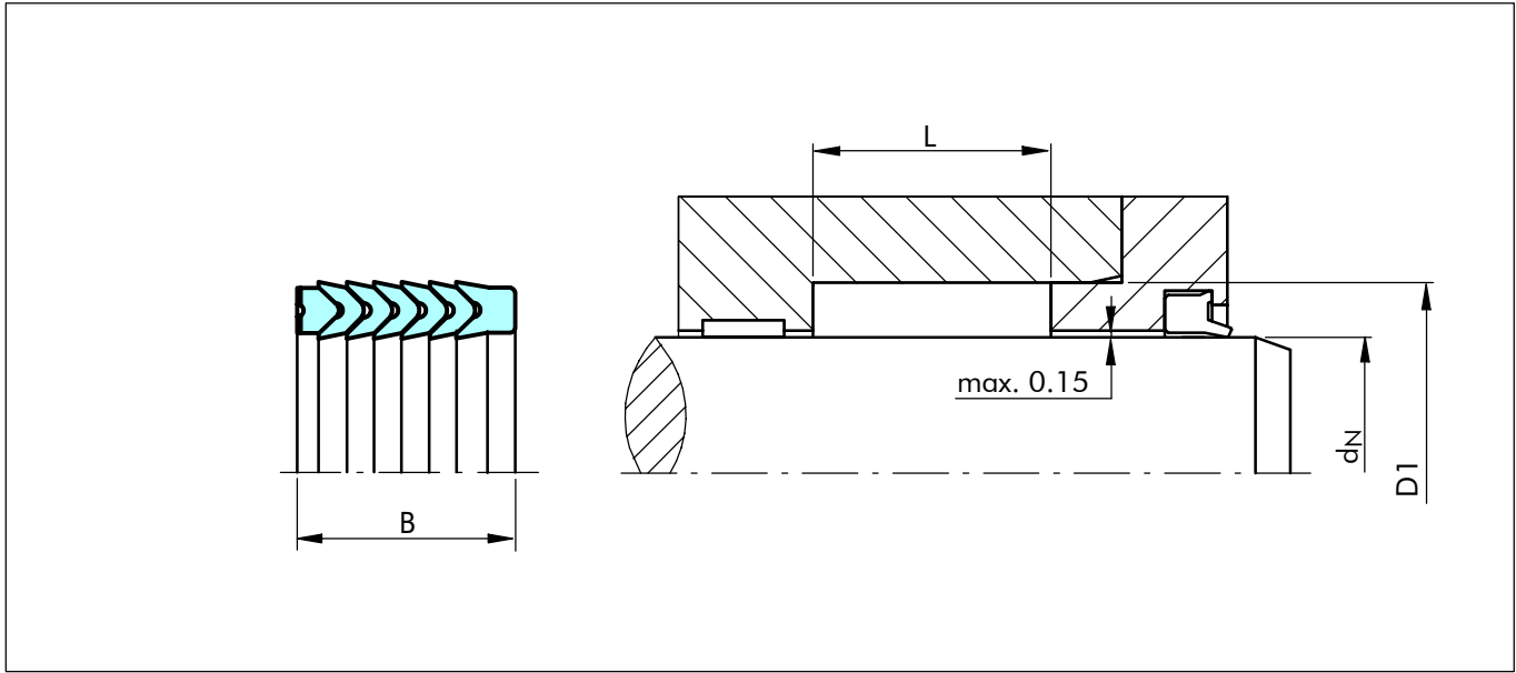
Figure 29 Installation drawing
