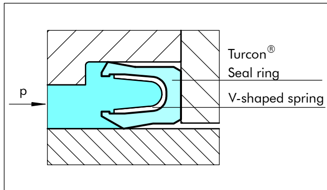
Figure 54 Turcon® Variseal® M2
