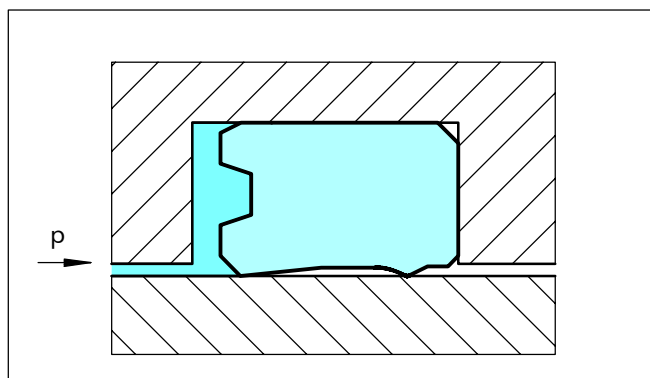
Figure 44 U-Cup, type RU2
