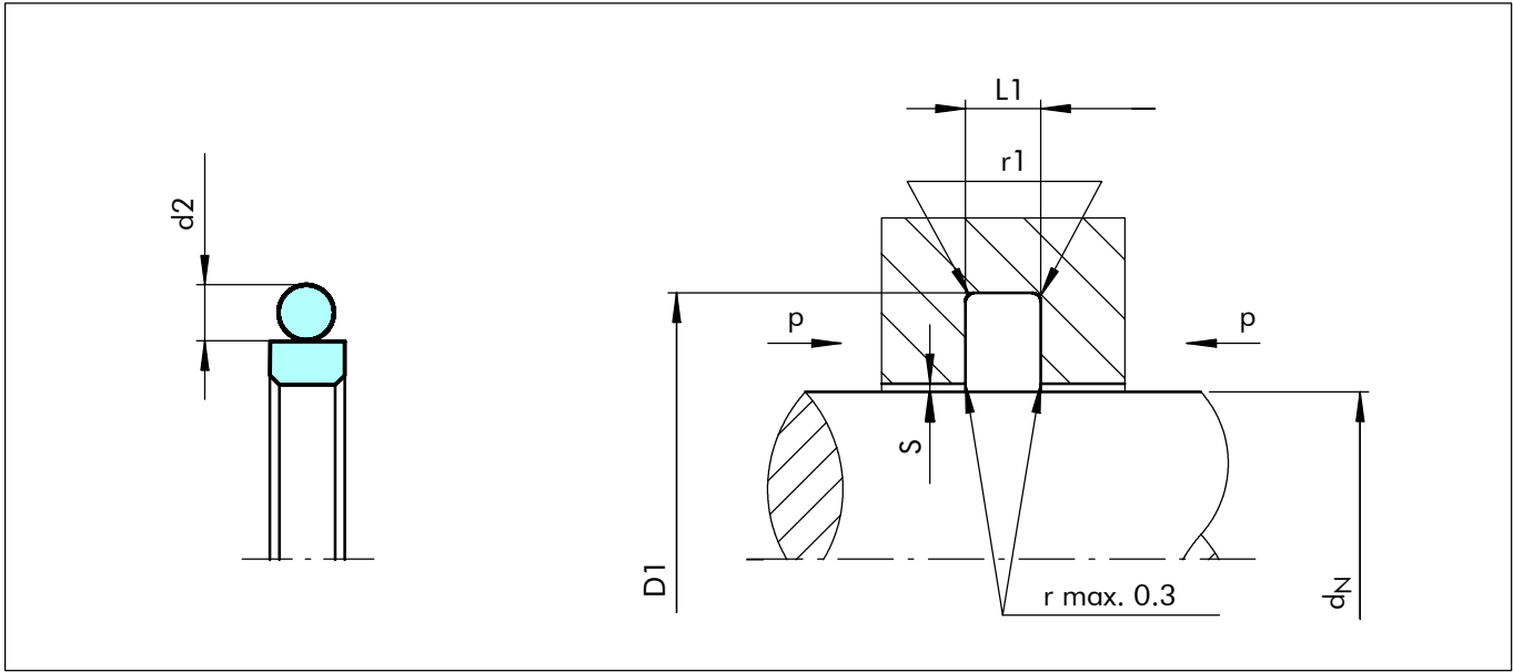
Figure 58 Installation drawing
