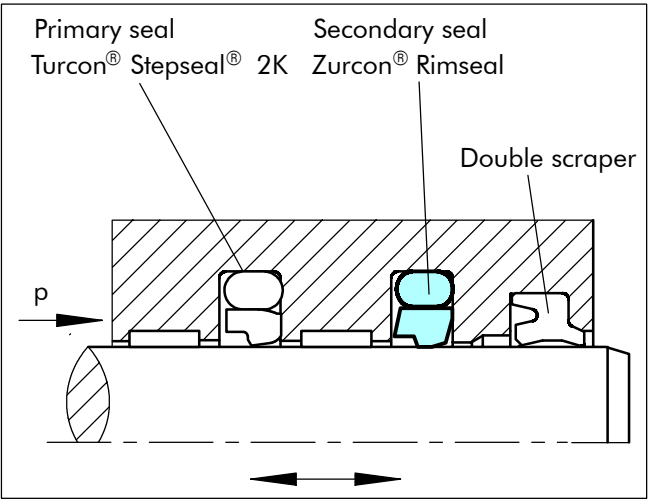
Figure 26 Zurcon® Rimseal in tandem configuration
