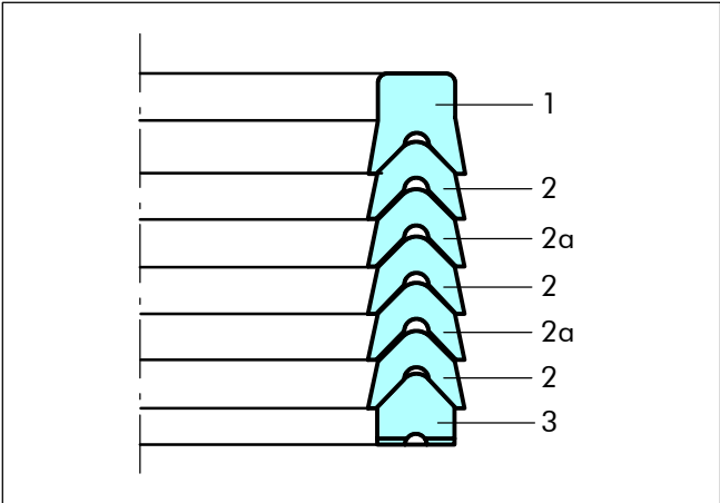
Figure 28 Veepac design
