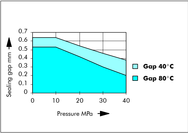
Figure 37 Sealing gap
