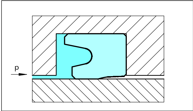
Figure 40 U-Cup, type RU0
