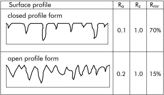
Figure 4 Profile forms of surfaces
