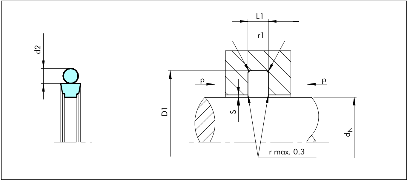
Figure 60 Installation drawing
