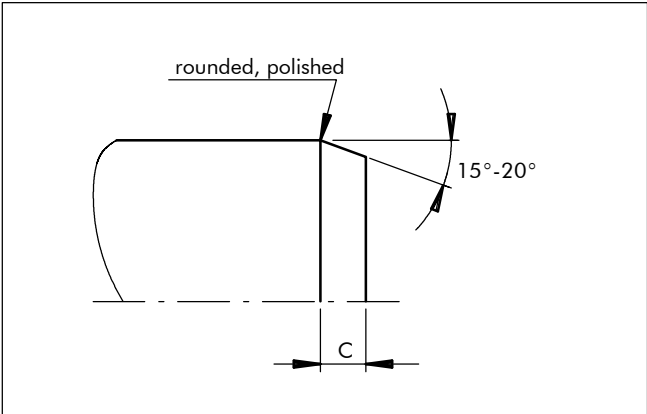
Figure 38 Lead-in chamfer
