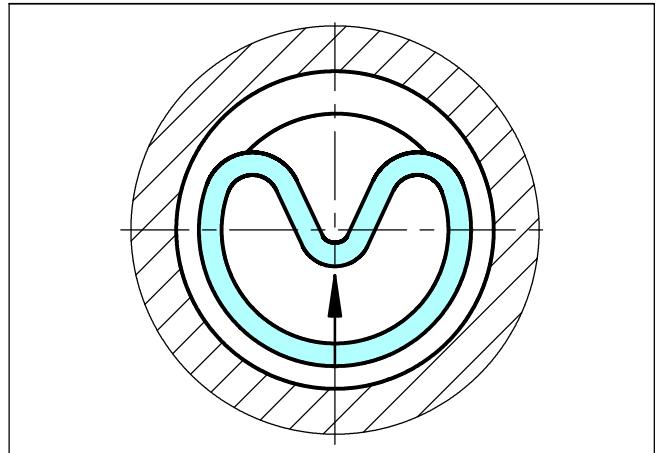
Figure 11 Inserting the seal ring into the closed groove
