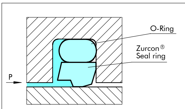
Figure 25 Zurcon® Rimseal
