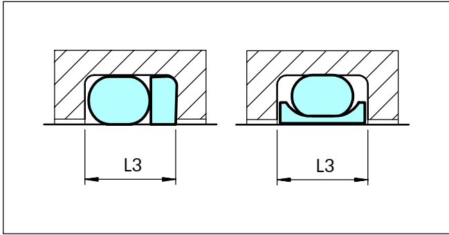
Figure 64 Groove width
