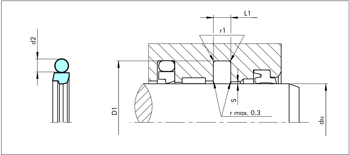
Figure 27 Installation drawing
