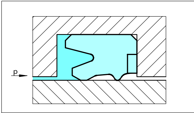
Figure 50 U-Cup, type RU3B
