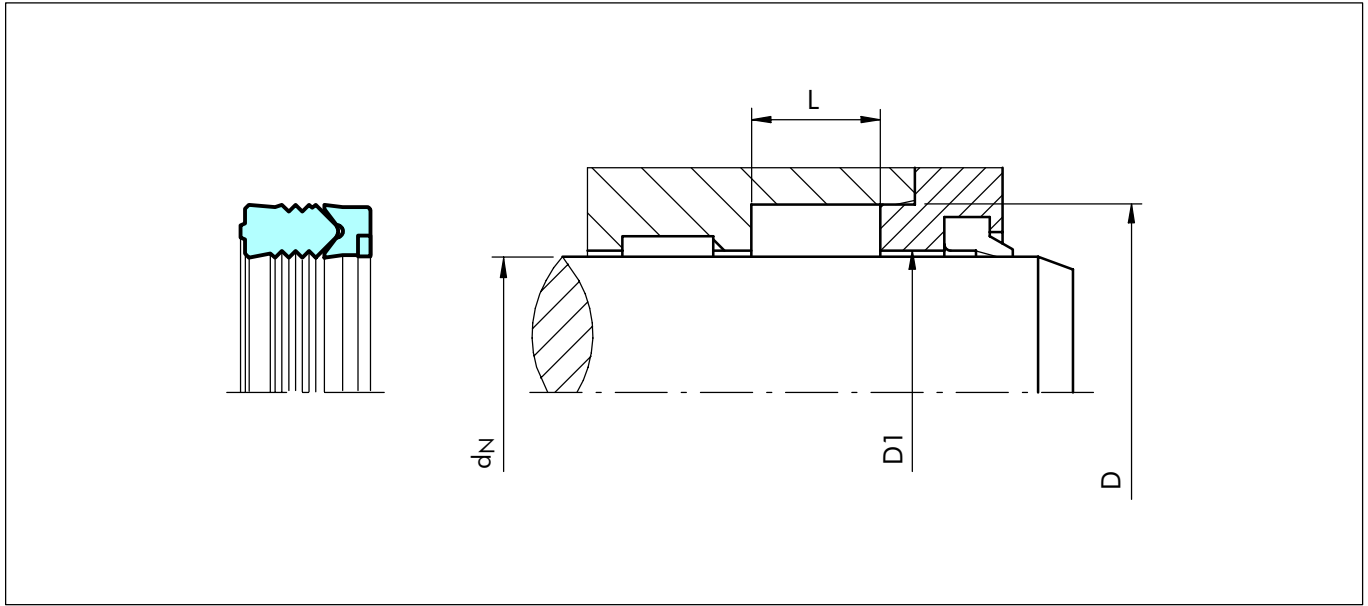
Figure 31 Installation drawing
