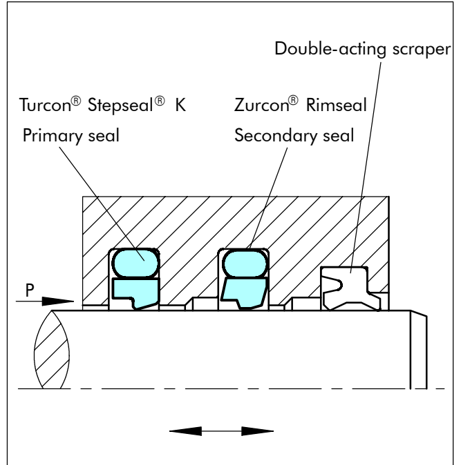
Figure 21 Turcon® Stepseal® K and Zurcon® Rimseal in tandem configuration
