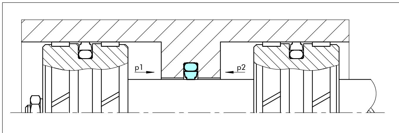
Figure 59 Turcon® Glyd Ring® T
