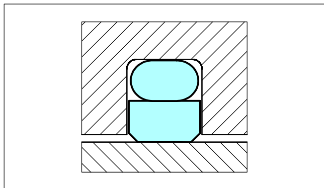
Figure 56 Turcon® Glyd Ring®
