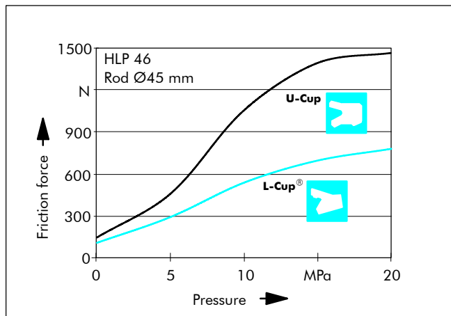
Figure 34 Friction dependent on pressure
