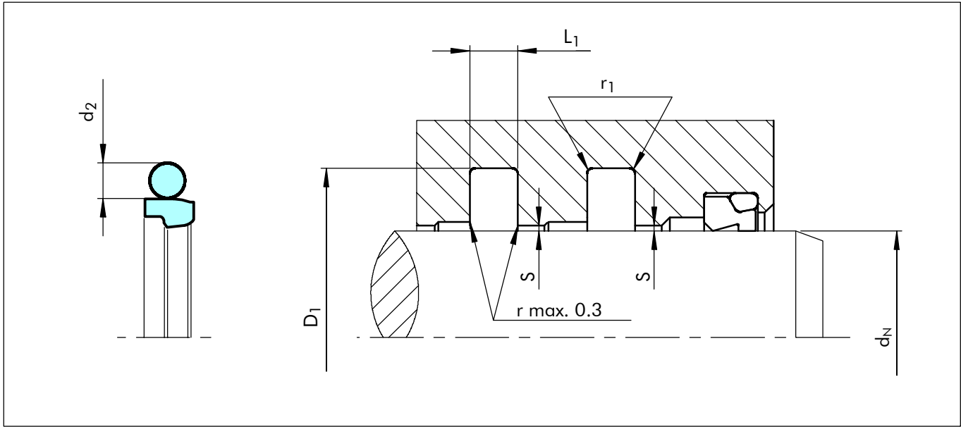
Figure 17 Installation drawing
