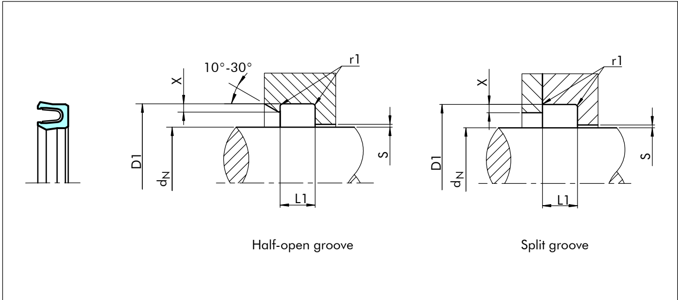
Figure 55 Installation drawing
