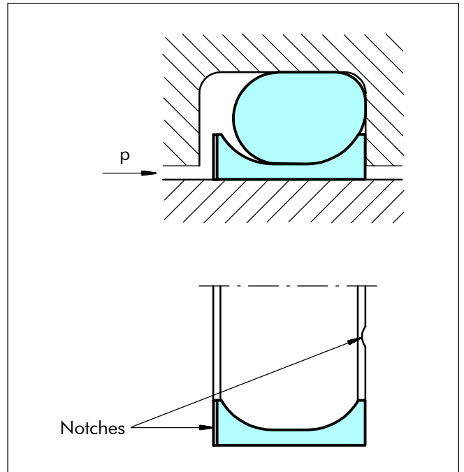
Figure 62 Turcon® Double Delta® with notches
