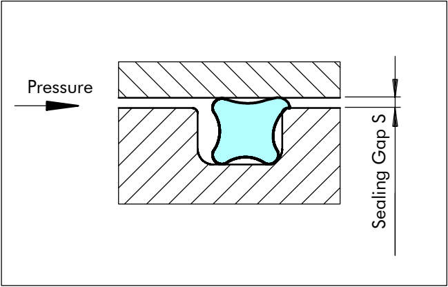
Figure 9 Extrusion gap
