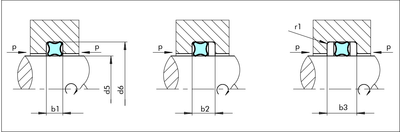
Figure14 Installation drawing
