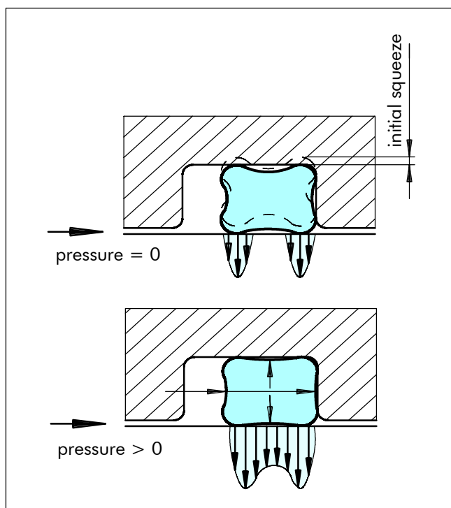
Figure 3 Sealing force with and without system pressure
