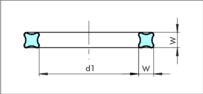
Figure11 QUAD-RING® Seal
