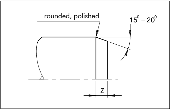
Figure 8 Lead-in chamfer for rods, shafts
