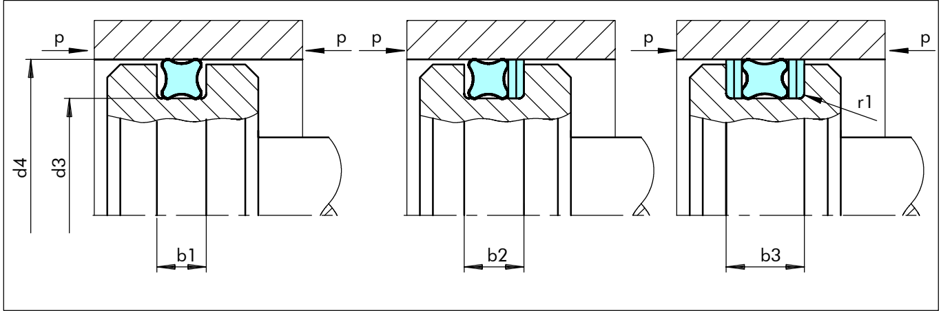
Figure12 Installation drawing
