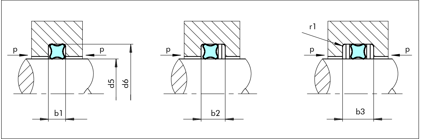
Figure13 Installation drawing
