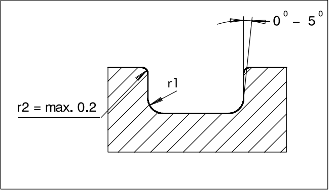
Figure 6 Groove design
