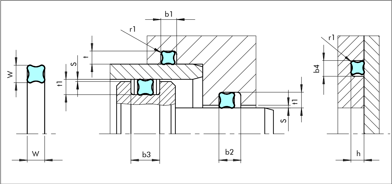
Figure 10 Installation drawing
